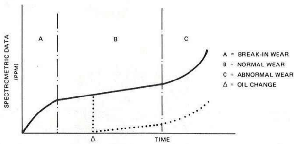
Figure 3. Typical Profile Small Particles
