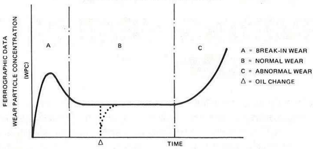
Figure 4. Typical Profile Large Particles
