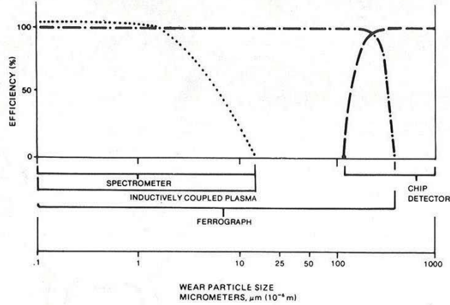
Figure 2. Particle Size vs Measurement Efficiency of Four Wear Monitoring Instruments
