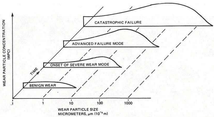
Figure 1. Typical Progression of Severe Wear
